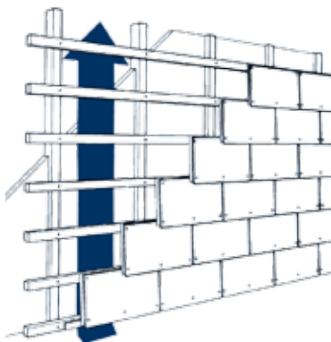
horizontale dekking (halfsteensverband)
